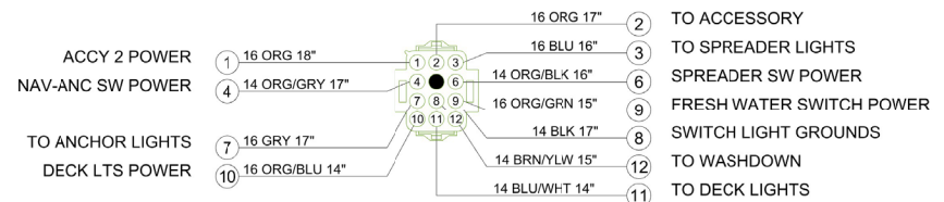
A 12 POS 15A MNLII FEMALE CAP W/SM PINS 052-2035 (11) 052-3017 14-16GA
