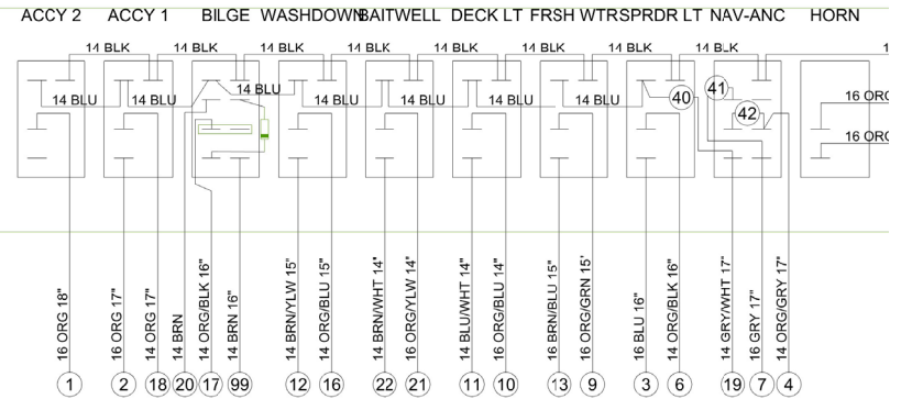
A 12 POS 15A MNLII FEMALE CAP W/SM PINS 052-2035 (11) 052-3017 14-16GA
