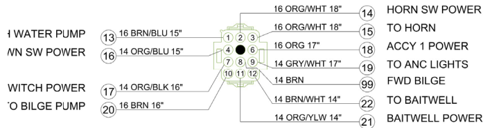
B 12 POS 15A MNLII FEMALE CAP W/SM PINS 052-2035 (10) 052-3017 14-16GA
